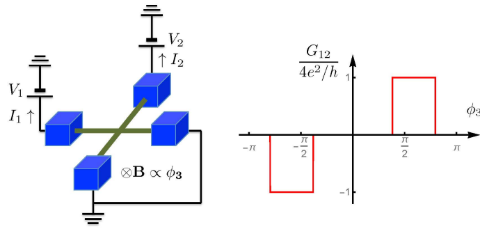
Figure: Left: setup of a multi-terminal Josephson junction between superconducting leads (blue) connected through a normal region (green). A magnetic field controls the superconducting phase difference between two of the leads, while two others are voltage-biased. Right: Quantization of the trans-conductance upon varying the superconducting phase difference
