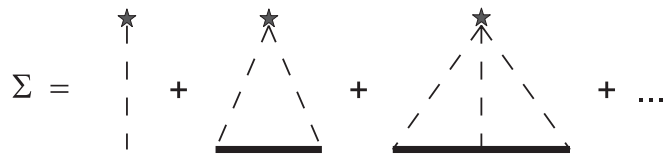
FIG. 1. Self-energy \Sigma(\mathbf{k}, \varepsilon) corresponding to the self-consistent T -matrix approximation. The scattering on a single impurity (dashed lines) is treated in all orders of the perturbation series. The self-consistency is achieved by inserting the bold lines for the Green functions, which means that they are calculated with the help of the presented self-energy.
