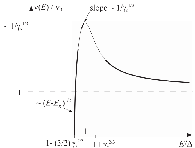
FIG. 3. Schematic (not numerically exact) DoS for a superconductor in the AG regime with a small concentration of magnetic impurities. The bold sectors of the curve are known analytically.
